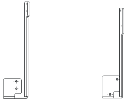
Figure 8: 6" & 8" Valve IP67 Switch Bracket
